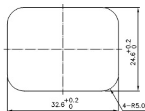
MOUNTING CUTOUT PANEL THICK : 1.5 mm
