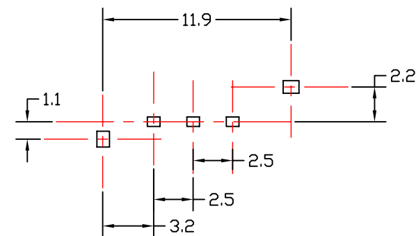
P. C. B TERMINAL POSITION
